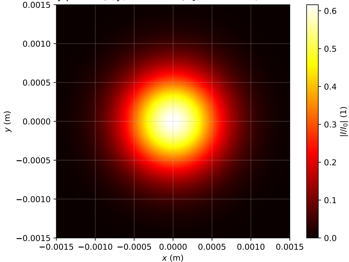
Intensity profile I(x, y, z = 1.911m)/I_0 , P_{in}=0.2P_{cr} , artificial time
